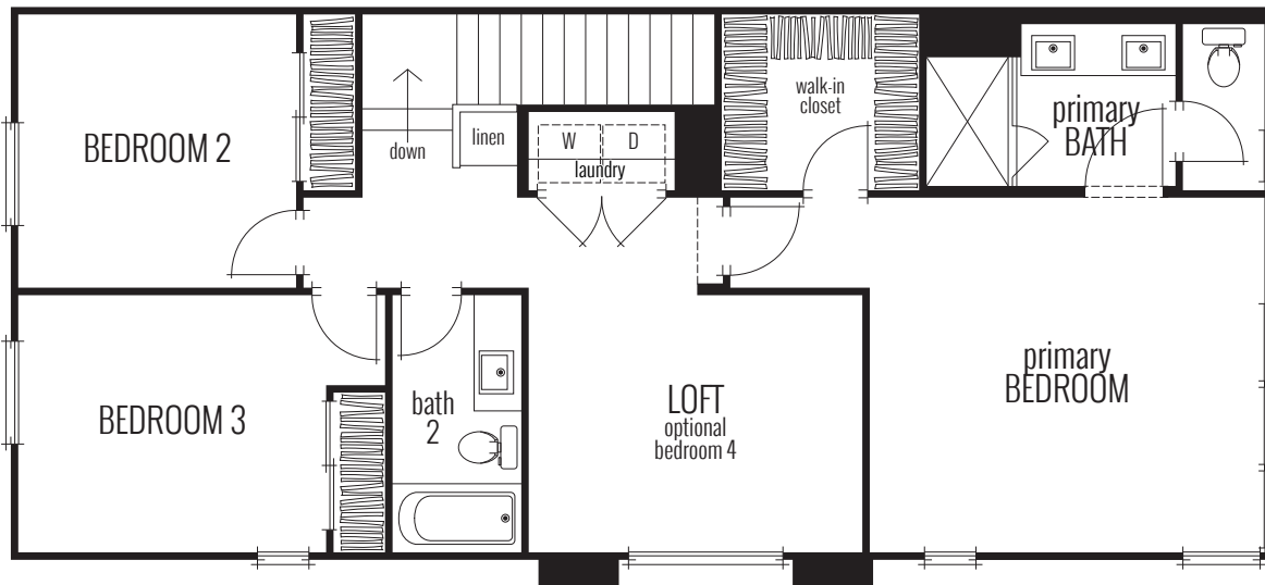
SECOND FLOOR
